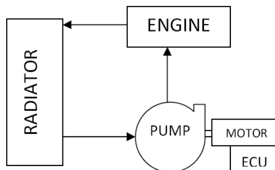
Fig. 9 Block diagram of cooling circuit
