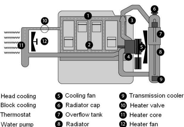
Fig. 1 Cooling System
