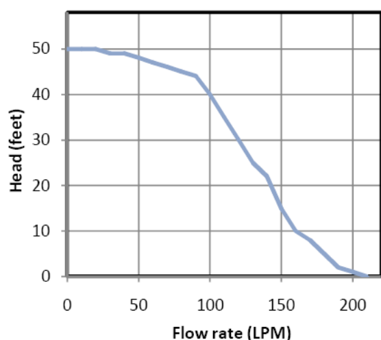
Fig. 7 Flow rate Vs Head
