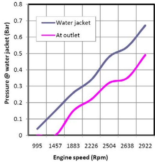
Fig. 4 Engine Speed Vs Pressure
