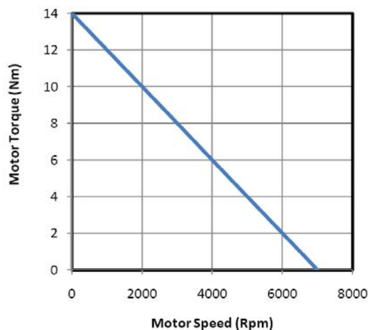
Fig. 10 Motor speed Vs Motor torque
