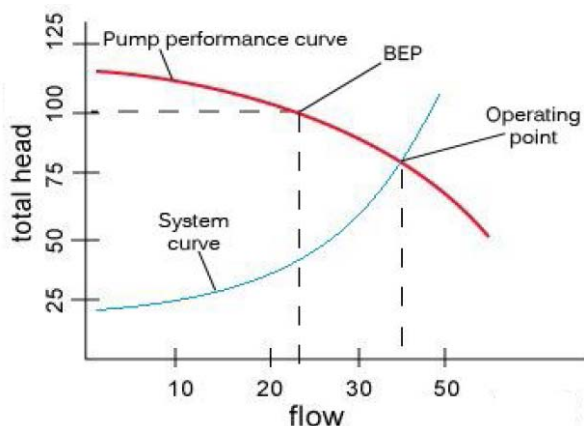
Fig. 6 System Curve
