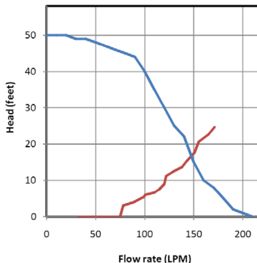
Fig. 8 Flow rate Vs Head/Water pump speed
