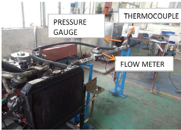
Fig. 3 Mechanical water pump test setup
