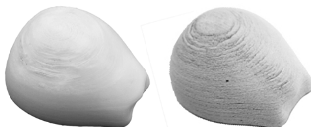
Fig. 6 Quality anomalies in a desktop FDM print (left) and inkjet salt print (right)
