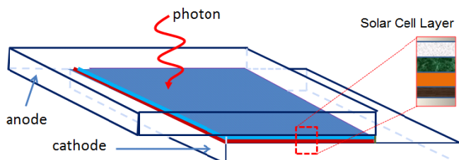
Fig. 2 Side view of DSSC structure
