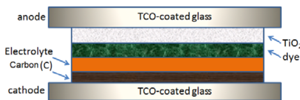
Fig. 1 Layer Structure of DSSC
