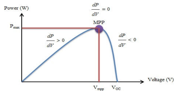
Fig. 5 Power voltage characteristic of solar panel
