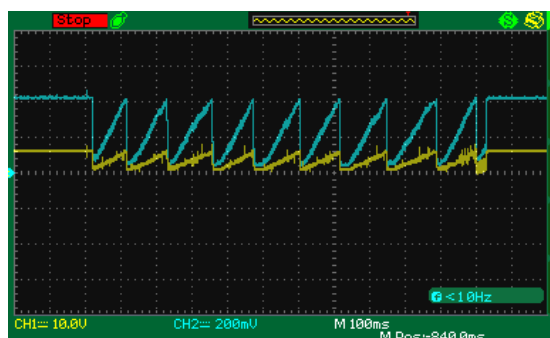
Fig. 10 Failure MPPT condition ( R_{load}=2\Omega )
