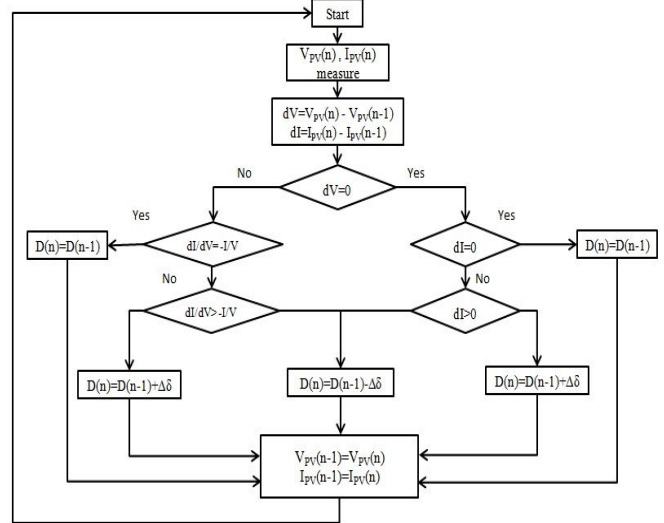
Fig. 4 Inc-Cond algorithm
