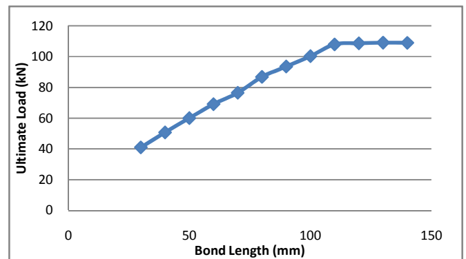
Fig. 3 Load vs. bond length for the quasi-static specimens
