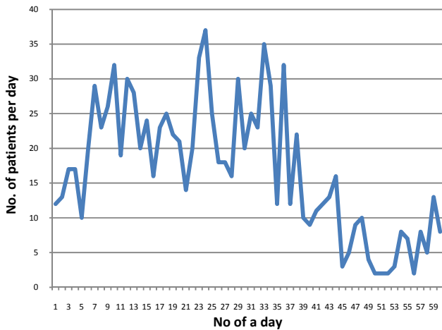
Fig. 1 Patients arrival pattern per day
