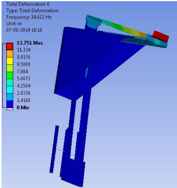
Fig. 13 Sixth mode shape of existing computer mount
