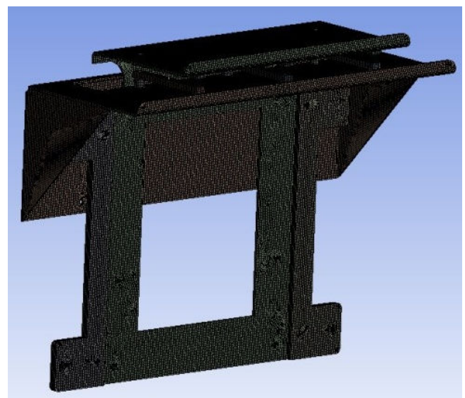
Fig. 8 Meshed computer mount
