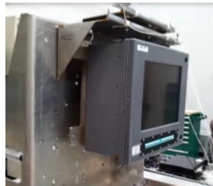
Fig. 14 Experimental setup for modal testing
