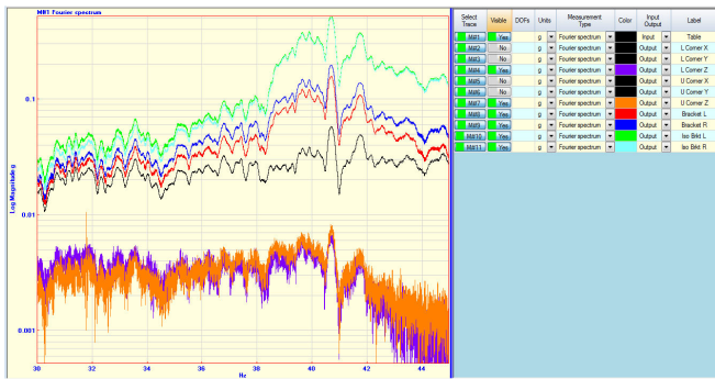
Fig. 15 Zoomed in results from 30 to 45 Hz
