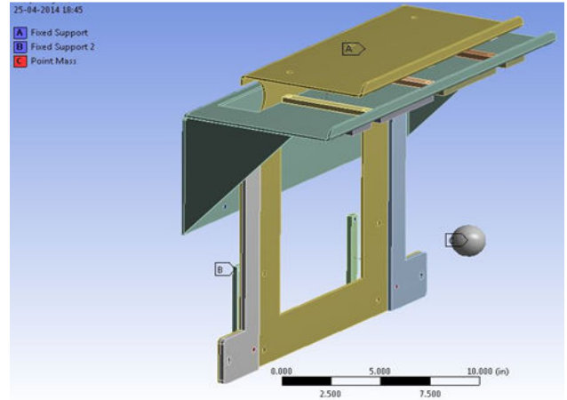
Fig. 11 Boundary Condition 3 for modal analysis
