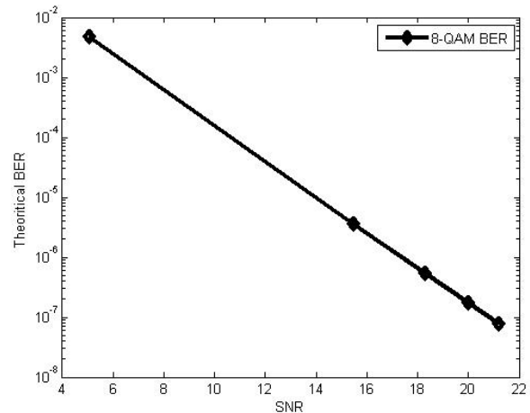
Fig. 11 BER and SNR of performance of 8-QAM
