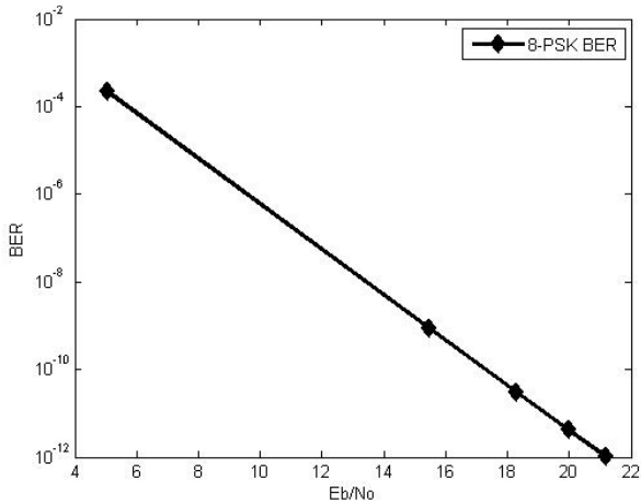
Fig. 7 BER and SNR performance of 8-PSK
