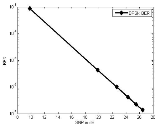
Fig. 2 BER and SNR performance of BPSK
