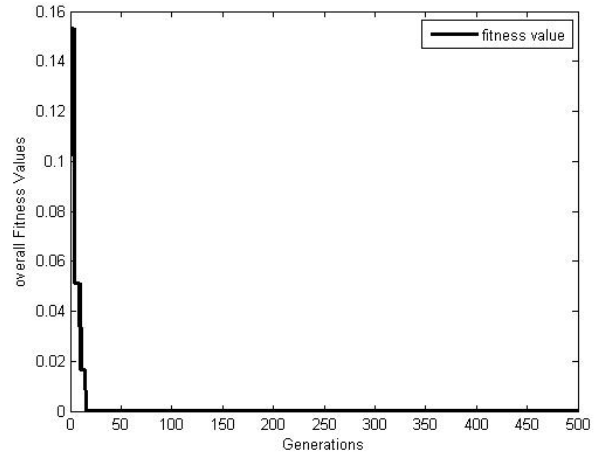
Fig. 15 Overall fitness value of BER for WLAN from 8-QAM
