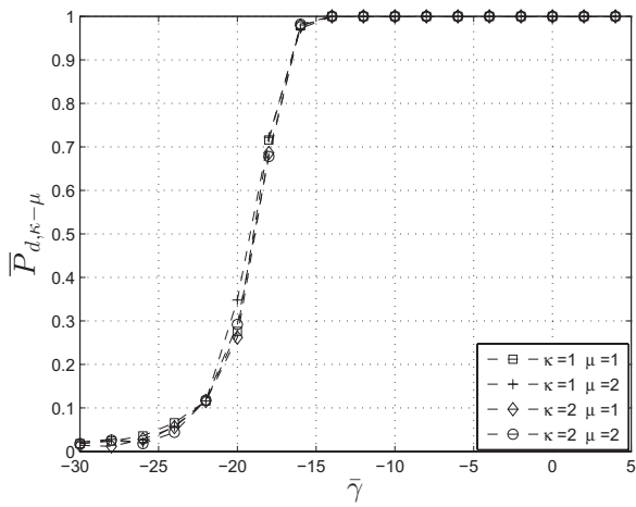
Fig. 4 \bar{P}_{d,\kappa-\mu} vs Avg.SNR( \bar{\gamma} ) for 2 \times 1 system
