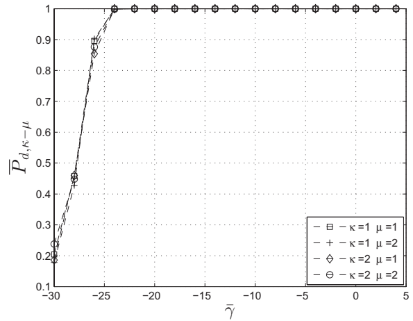
Fig. 7 \bar{P}_{d,\kappa-\mu} vs Avg.SNR( \bar{\gamma} ) for 4 \times 4 system
