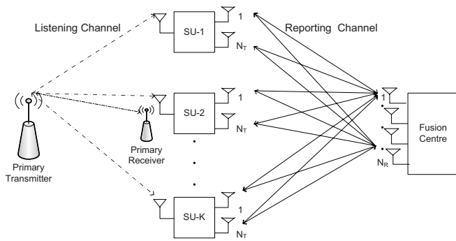
Fig. 1 Cooperative-MIMO reporting network
