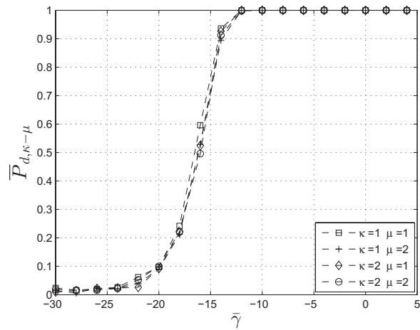
Fig. 2 \bar{P}_{d,\kappa-\mu} vs Avg.SNR( \bar{\gamma} ) for 1 \times 1 system
