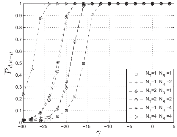
Fig. 8 \bar{P}_{d,\kappa-\mu} vs Avg.SNR( \bar{\gamma} ) for \kappa = 2, \mu = 2
