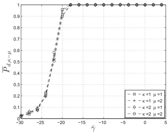
Fig. 6 \bar{P}_{d,\kappa-\mu} vs Avg.SNR( \bar{\gamma} ) for 1 \times 4 system
