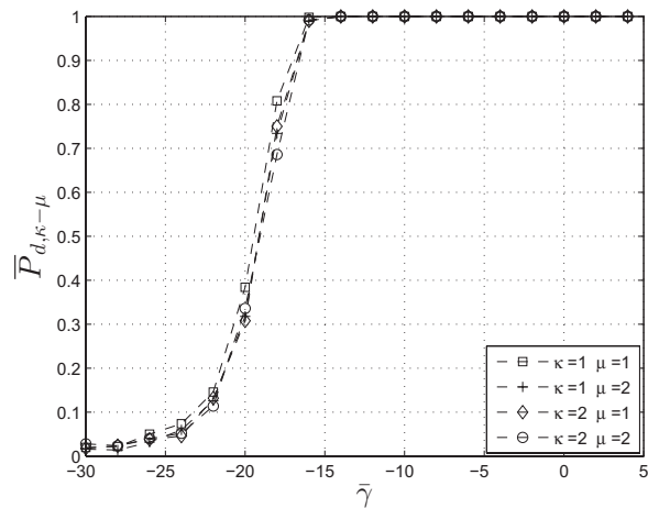
Fig. 3 \bar{P}_{d,\kappa-\mu} vs Avg.SNR( \bar{\gamma} ) for 1 \times 2 system
