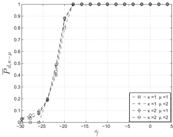
Fig. 5 \bar{P}_{d,\kappa-\mu} vs Avg.SNR( \bar{\gamma} ) for 2 \times 2 system
