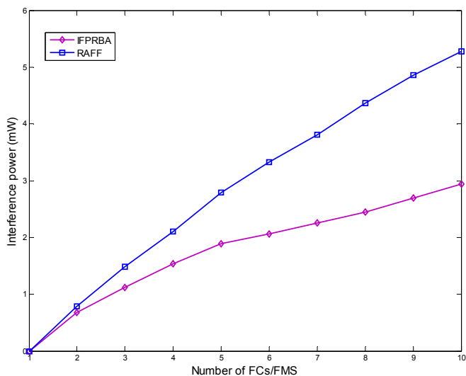
Fig. 4 Overall interference power experience by 10 femtocells/FMS
