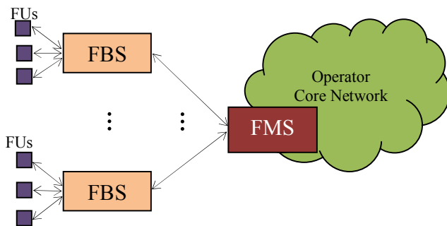
Fig. 1 Femtocell Network Architecture
