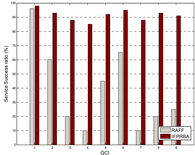
Fig. 3 Service success ratio comparison between existing RAFF and IFPRBA algorithm for various QCI
