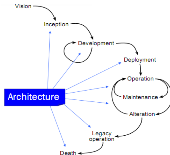
Fig. 1 Software Life Cycle [5]
