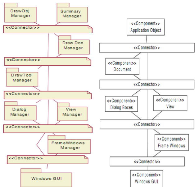
Fig. 6 Prescriptive vs. Descriptive Architecture [14]
