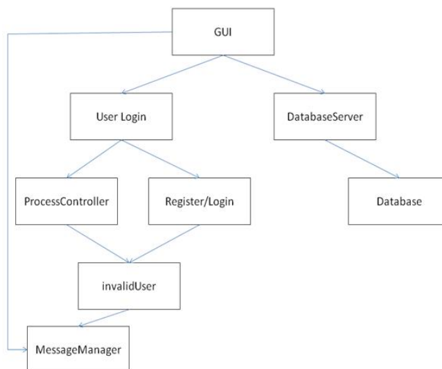
Fig. 10 Architecture after removal of dependency
