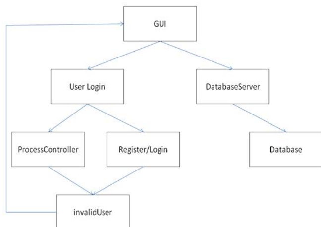
Fig. 9 A cycle sneaks in
