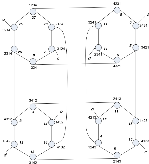
Fig. 4 4-Star network – load balancing phase 1-A
