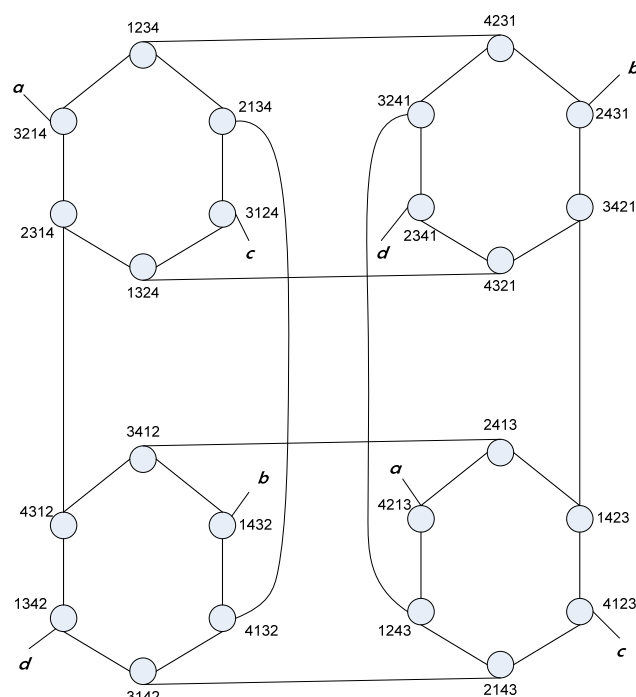
Fig. 1 The 4-Star Graph
