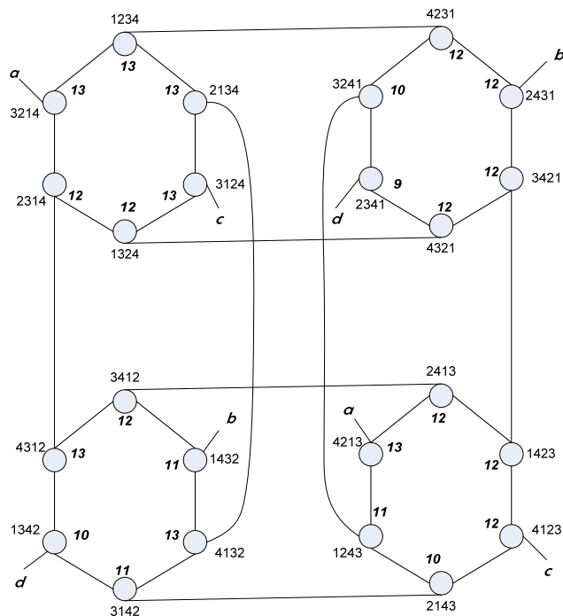
Fig. 7 4-Star network –load balancing – phase 2
