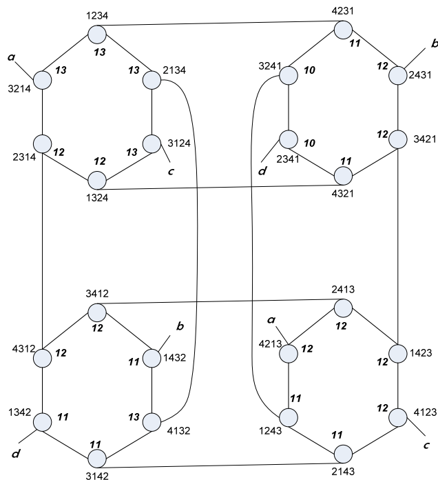
Fig. 8 4-Star network – load balancing – phase 3
