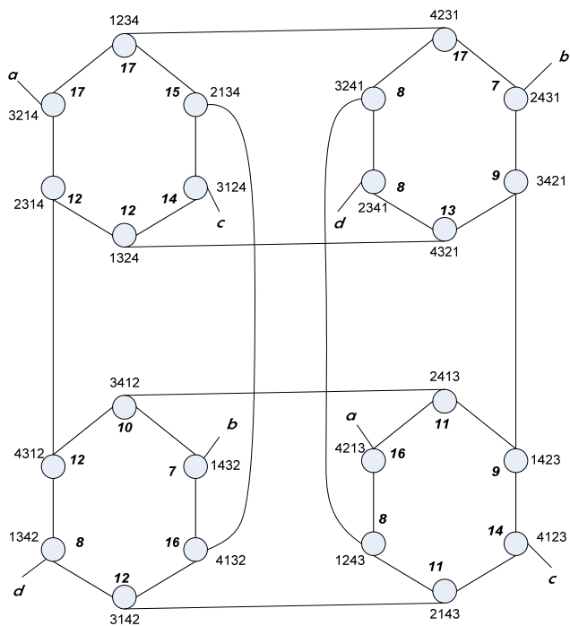
Fig. 6 4-Star network – load balancing phase 1-C
