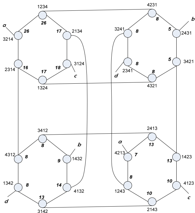
Fig 5 4-Star network – processors load balancing phase 1-B
