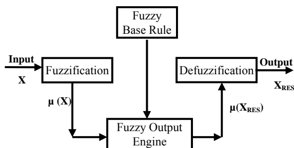
X: the input vector, X_{RES} : the input commands, \mu(x) and \mu(X_{RES}) : the correspond memberships functions
