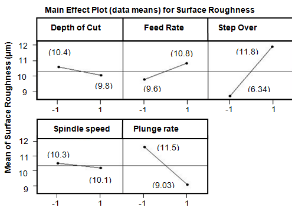
Fig. 6 Graph of the significance of machining parameters
