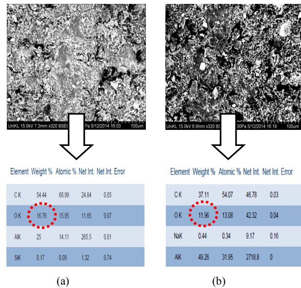
Fig. 5 SEM-EDX imaging and chemical content of (a) machining with coolant (b) machining without coolant Notes: 1) "K" - K shell energy level 2) Weight % - Ratio of the weight of the element to the weight of the sample 3) Atomic % - Ratio of the number of atoms of the element to the total number of atoms in the sample 4) Net Int. - Average intensity of X-ray in kilo count per second (kcps)
