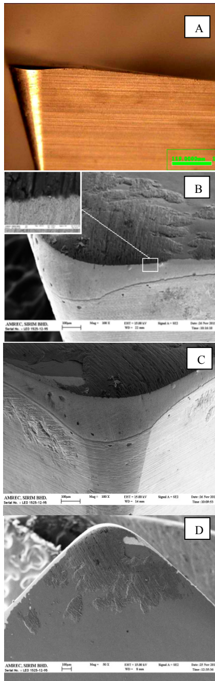
Fig. 5 Tool wear TiB 2 insert, optic (a) before cutting. it was observed using a Sometech SV-35 video microscope and SEM image of the flank view, (b) - 200µm, nose view, (c)-100µm and top view, (d) - 100µm, showing the deformation of wear at 123.2 min for 370 m/min cutting speed, feed rate 0.8 m/tooth and doc 0.4mm.
