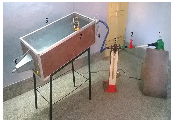
Fig. 2 Experimental setup of solar air collector system
