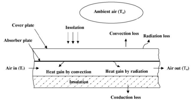
Fig. 1 Energy balance of solar air heater [16]
