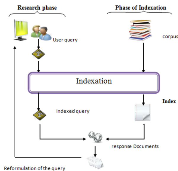
Fig. 1 Process of Information Retrieval
