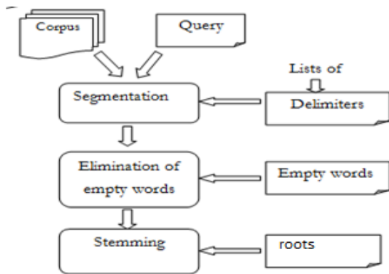
Fig. 4 Phases of indexing of proposed system
