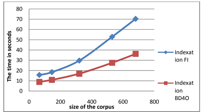
Fig. 5 Comparison of indexing time in db4o and the inverted file
