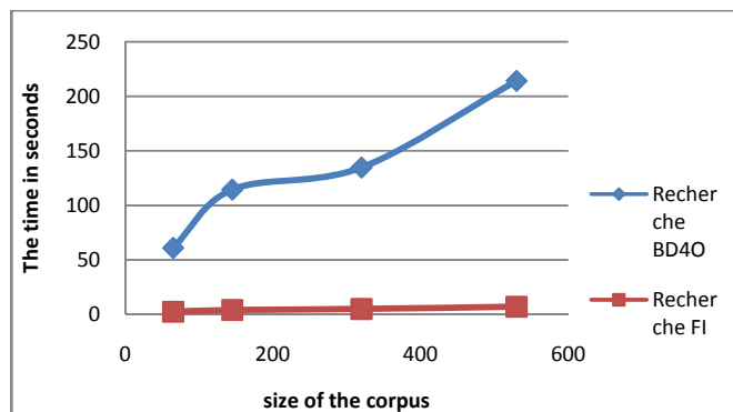
Fig. 7 Comparison of search time in the BD4O and FI size of the corpus
