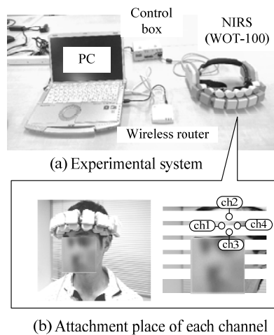
Fig. 1 Experimental system
