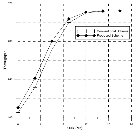
Fig. 5 The throughput performance of the conventional and proposed scheme
