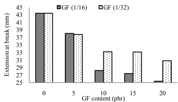
Fig. 10 Extension at break of PVC-GF foam composites
