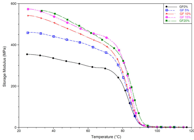
Fig. 6 (b) Storage Modulus ( E' ) for 1/32" GF
