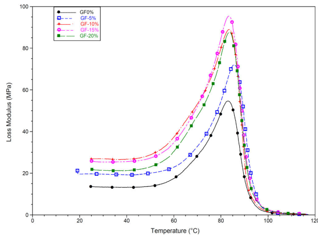
Fig. 7 (a) Loss Modulus ( E'' ) for 1/16" GF
