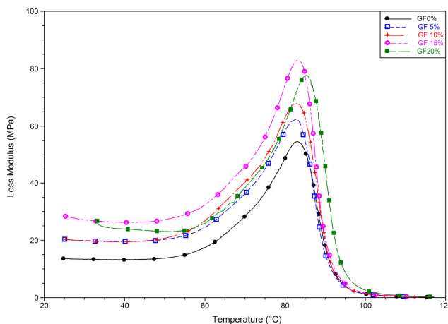
Fig. 7 (b) Loss Modulus ( E'' ) for 1/32" GF
