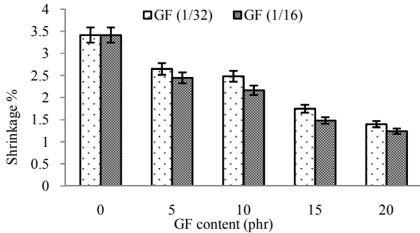
Fig. 4 Dimensional stability of PVC-GF foam composites
