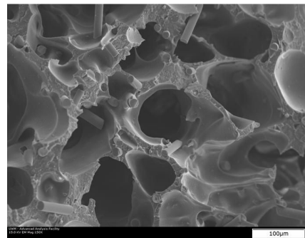
Fig. 2 SEM micrographs at 150x of 1/32" 15% GF-PVC
