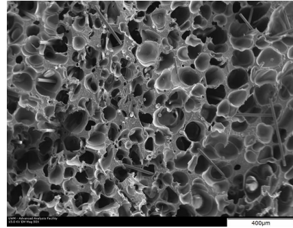
Fig. 1 SEM micrographs at 50x of 1/16" 15% GF-PVC
