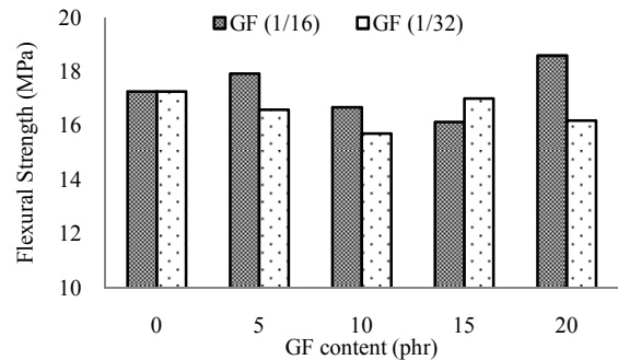
Fig. 9 Flexural strength of PVC-GF foam composites
