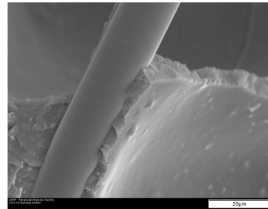
Fig. 3 SEM image at 1000x of GF interface with PVC foam
