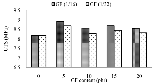
Fig. 8 Ultimate tensile strength (UTS) PVC-GF foam composites
