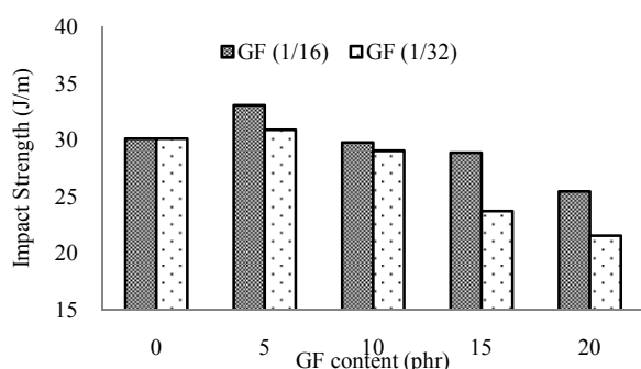
Fig. 11 Impact strength of PVC-GF foam composites
