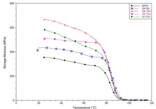
Fig. 6 (a) Storage Modulus ( E' ) for 1/16'' GF
