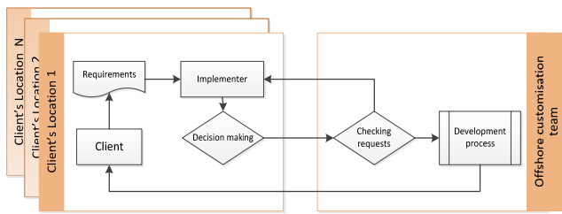
Fig. 3 CCRD model — local decision making
