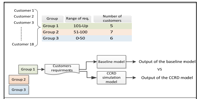
Fig. 5 Evaluation of experiment design using the Black-Box comparison approach
