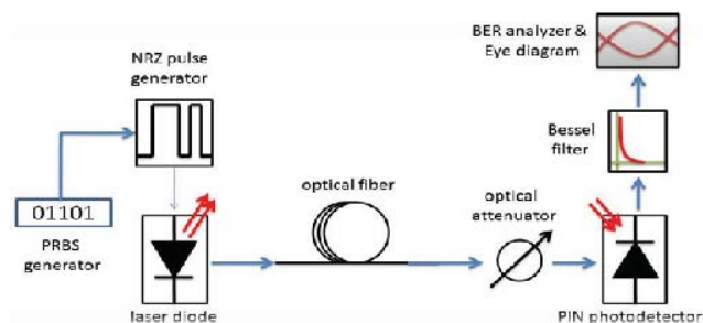
Fig. 1 Scheme of the designed fiber communication system
