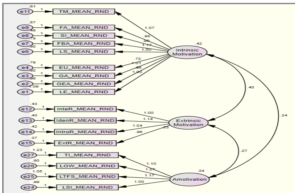
Fig. 1 CFA for Variables with Relations
