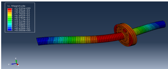
Fig. 3 2 nd mode shapes Freq = 0.48805Hz → U_{max}=1.035mm
