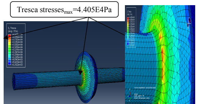
Fig. 7 Representation of Tresca stress
