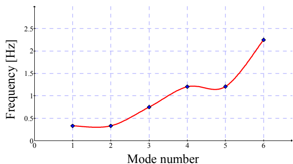
Fig. 9 Frequency function in mode number
