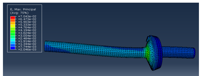
Fig. 8 Representation of the strain distribution
