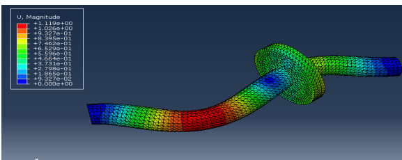
Fig. 4 5 th mode shapes, Freq = 1.4024 Hz → U_{max}=1.119mm
