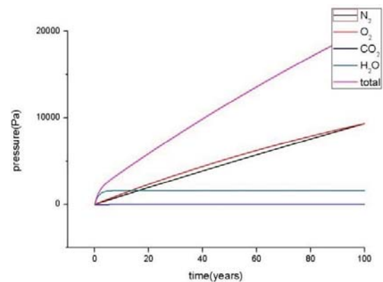
(b) Three-layer Al-metallized envelope
