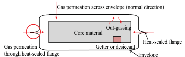
Fig. 2 Inner pressure increase factors
