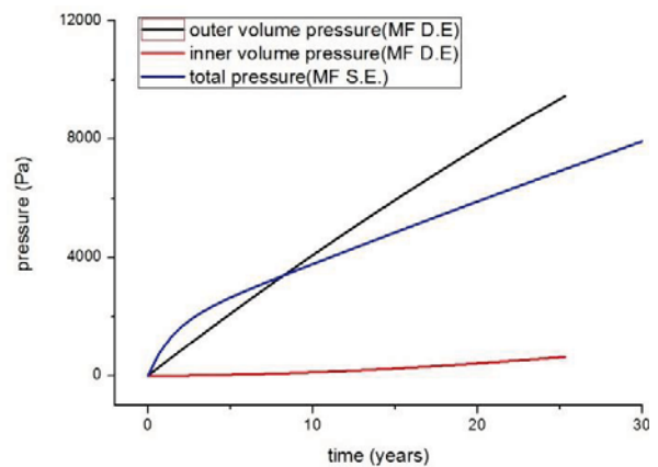
(b) Getter-inserted VIP
