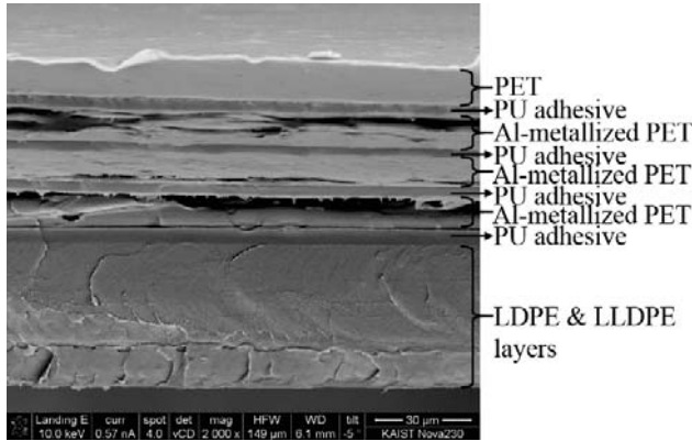
(a) Three-layer Al-metallized envelope
