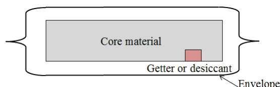
Fig. 1 General structure of the VIP
