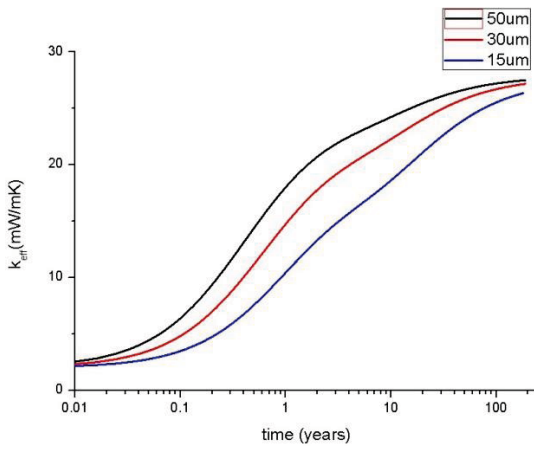
(b) Three-layer Al-metallized envelope
