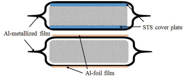
Fig. 7 Metal-barrier-added enveloping method
