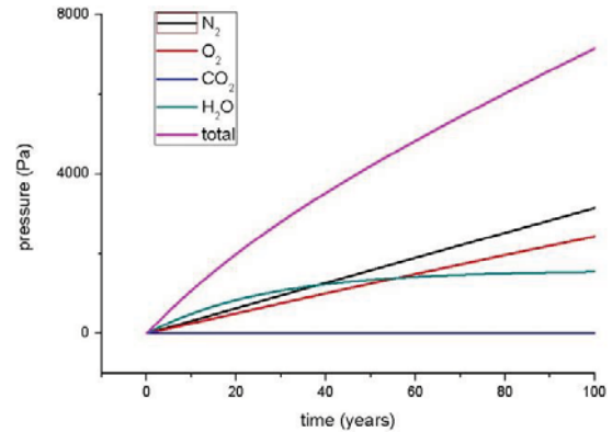
(a) Al-foil envelope
