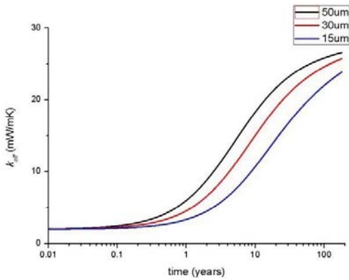
(a) Al-foil envelope
