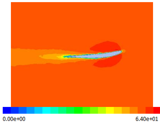
(a) Angle of attack = 0^{\circ}
