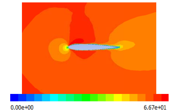
(c) Angle of attack = 4^\circ
