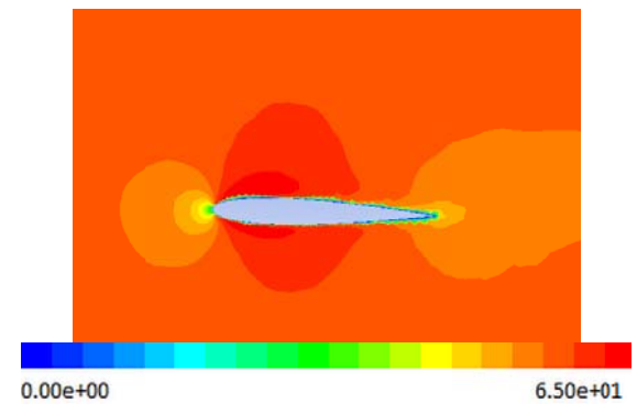
(b) Angle of attack = 2^\circ
