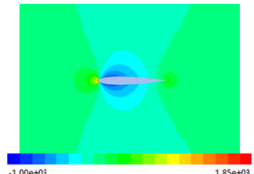
(a) Angle of attack = 0^\circ
