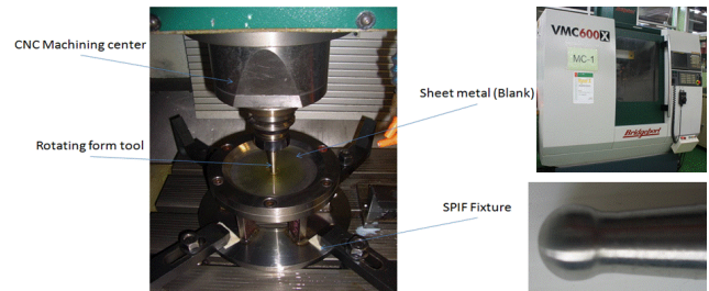
Fig. 4 The SPIF equipment, tool and CNC machine tool
