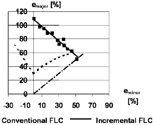
Fig. 3 Conventional FLC of AA1050 and Incremental FLC [3]
