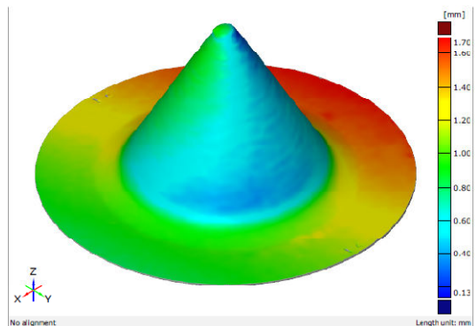
(a) SS 400 thickness distribution
