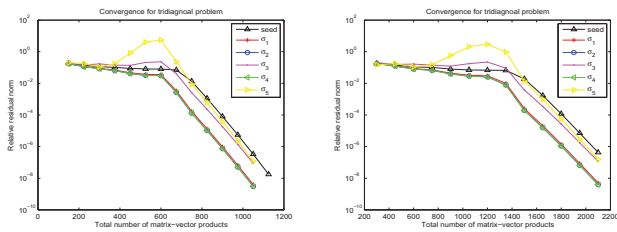
Fig. 1. Convergence history of GLGMRESIRsh for tridiagonal problem. Left: p = 5 , Right: p = 10 .
