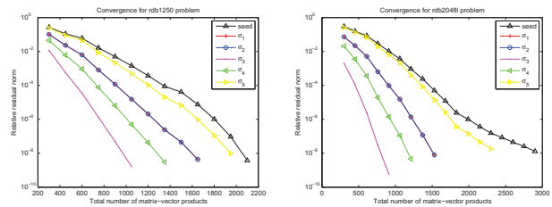
Fig. 2. Convergence history of GLGMRESIRsh for RDB1250 and RDB2048.
