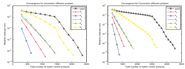
Fig. 3. Convergence history of GLGMRESIRsh for convection diffusion problem. Left: n = 16641 , Right: n = 66049 .
