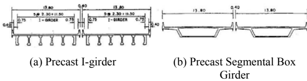
Fig. 5 Comparison between I-Girder and Box Girder superstructures
