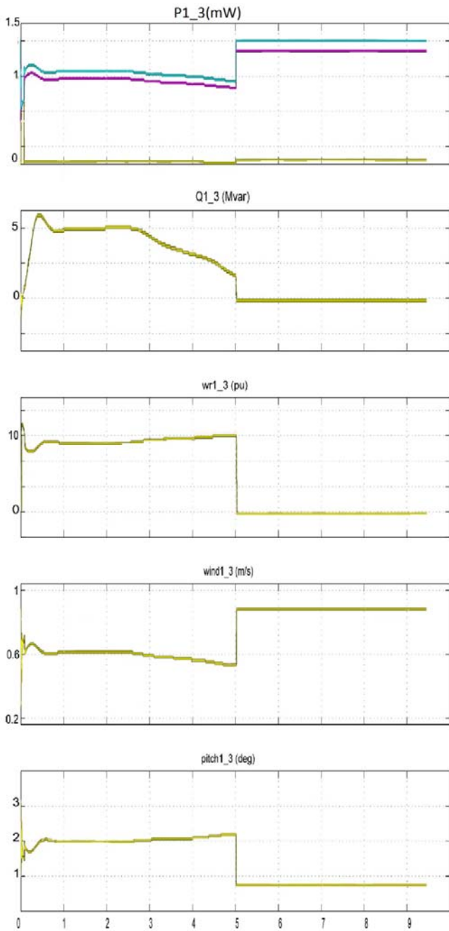
B) Curves for part load
