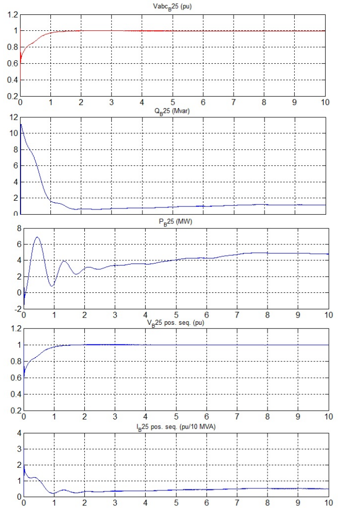
(b) Curves for part load
