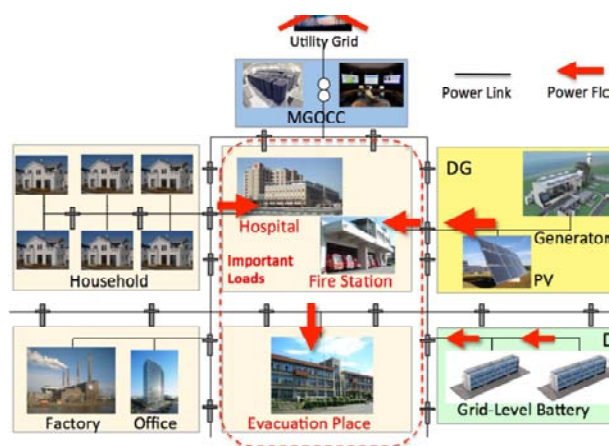
Fig. 1 Overview of the Priority of Load shedding
