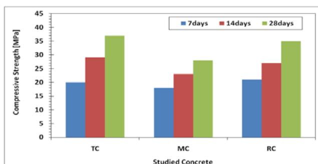
Fig. 8 Compression strength evolution as function type different of concrete (with adjuvant)
