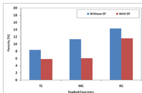
Fig. 9 Porosity of studied concretes
