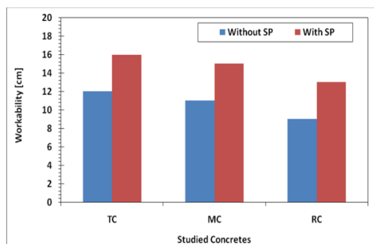
Fig. 6 Workability of concretes
