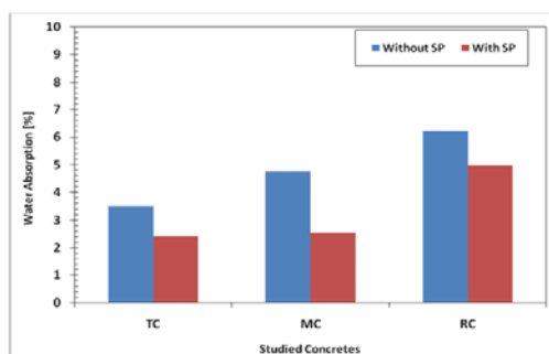
Fig. 10 Water absorption of studied concretes
