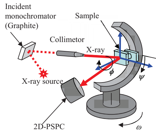
Fig. 3 Geometry of the diffractometer
