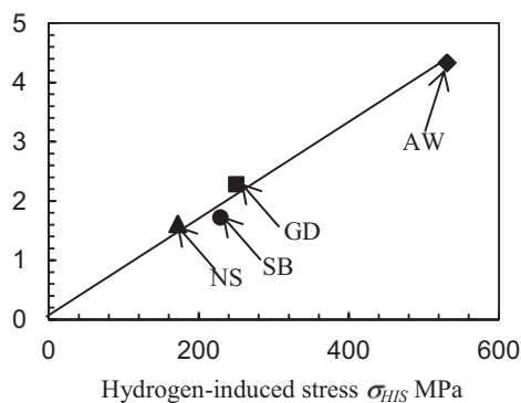
Fig. 9 Relationship between hydrogen content and hydrogen-induced stress
