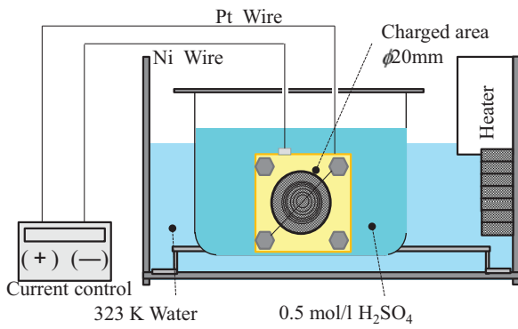
Fig. 1 Apparatus for the cathodic hydrogen charging
