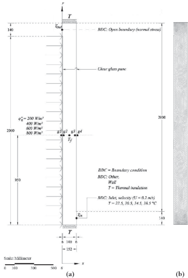
Fig. 3 Schematic diagram of the DCGW and DTGW
