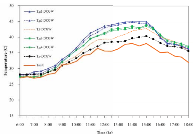
Fig. 4 Hourly variation of measured temperature of DCGW
