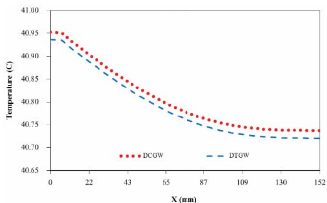
Fig. 8 Simulated result across the air gap temperature of DCGW and DTGW, q''=800 \text{ W} \cdot \text{m}^{-2} , T=38.5 \text{ C} , u=0.2 \text{ m} \cdot \text{s}^{-1}
