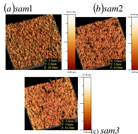
Fig. 1 AFM images of thin films with different percentage of carbon,
